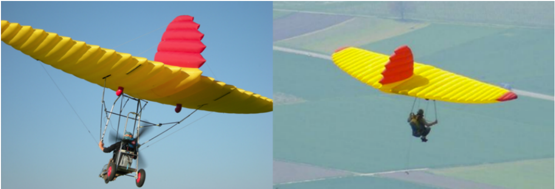
Figure 2. Woopy-Fly aircraft with inflatable wing. Similar to CGS Hawk, the inflatable wing has chordwise bumps and ridges which is hypothesized to affect the surface flow direction.
