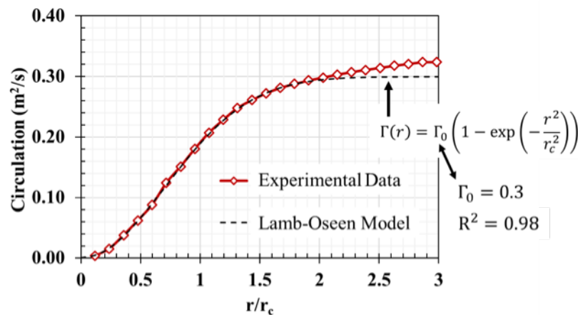
Figure 18. Determining total circulation of the wingtip vortex by fitting the experimental data with the Lamb-Oseen vortex model. The current graph is for the baseline NACA 0012 wing at 8^\circ angle of attack.
